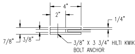
WALL MOUNTED GUIDE DETAIL
