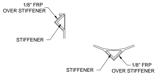
EMBEDDED STIFFENER DETAILS
