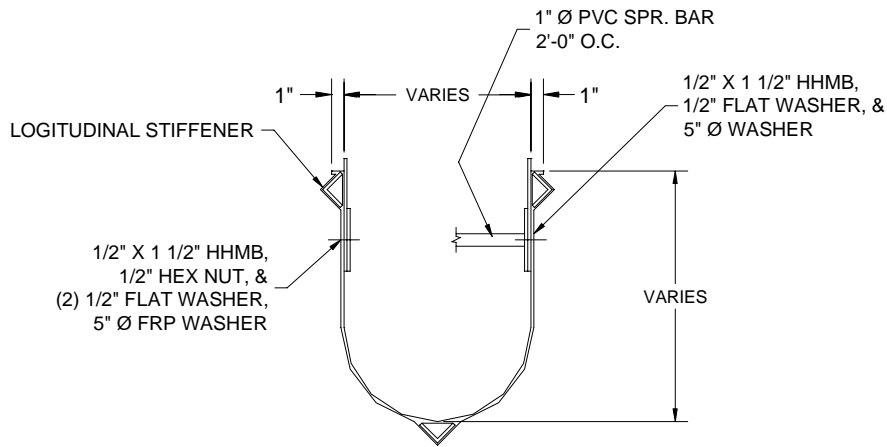
CROSS SECTION TROUGH
