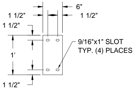
BAFFLE SPLICE PLATE DETAIL
