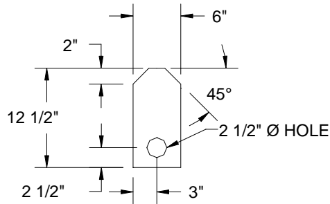
WEIR SPLICE PLATE DETAIL
